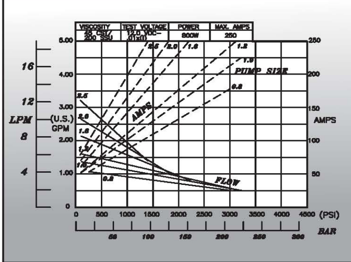
KM08 Flow/AMP vs. Pressure Curve
