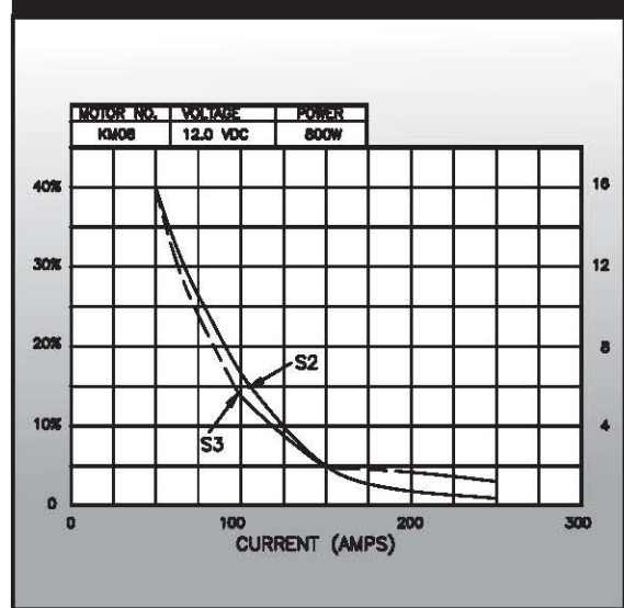
KM08 Motor Duty Cycle
